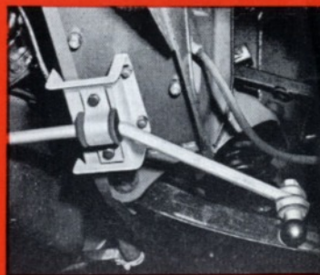
A.1 anti-roll bar fitted to A.35
