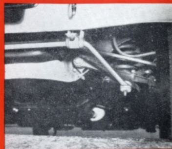
BMC.1 anti-roll bar fitted to A.55 Mark II, etc.
